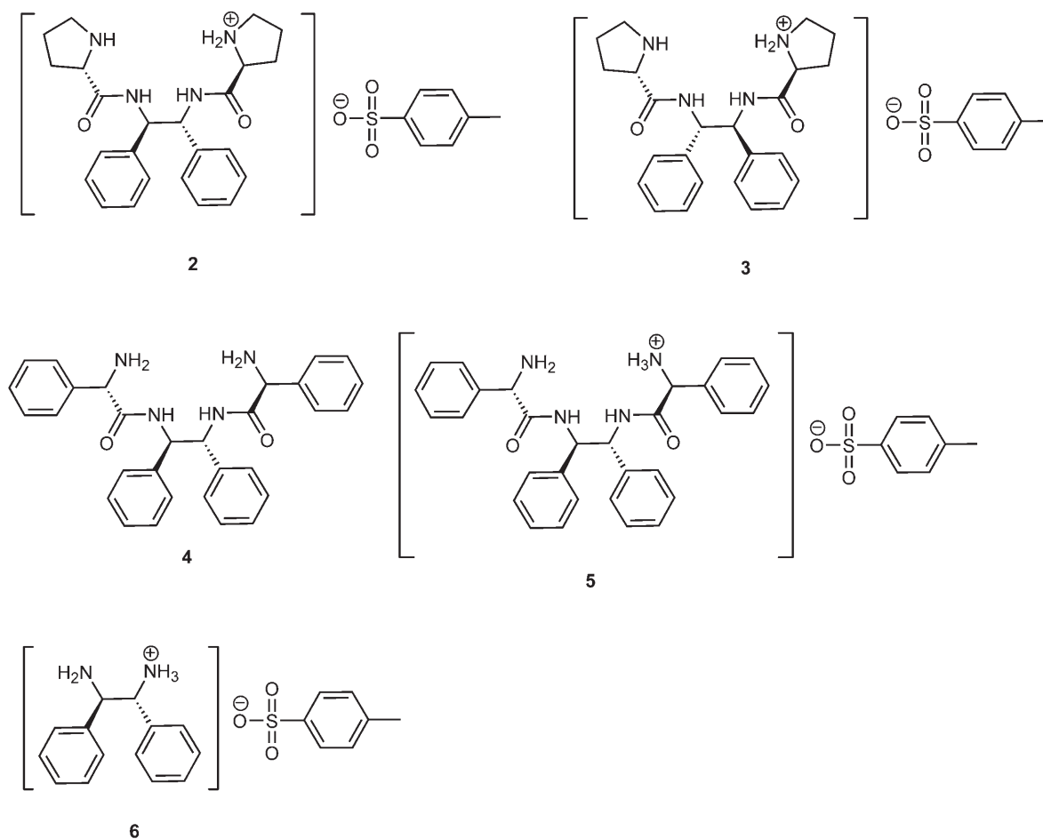
Figure 4. The evaluated chiral cation catalysts.
