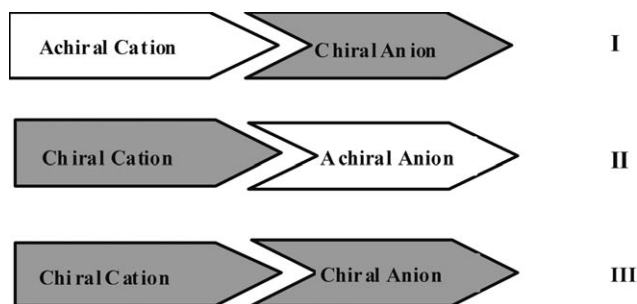
Figure 1. Combinations of chiral functional salts.
