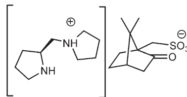
Figure 2. Barbas III's ammonium salt.
