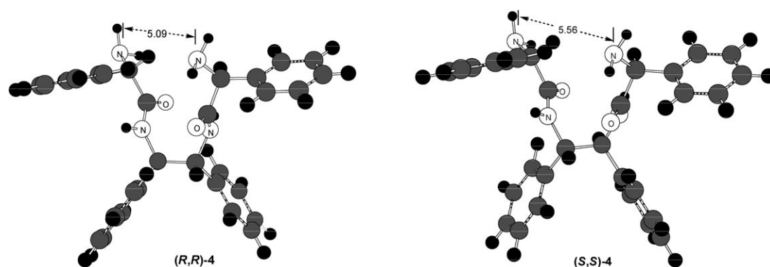
Figure 6. The optimized geometries of (R,R)-4 and (S,S)-4 at B3LYP/6-31G(d) level.
