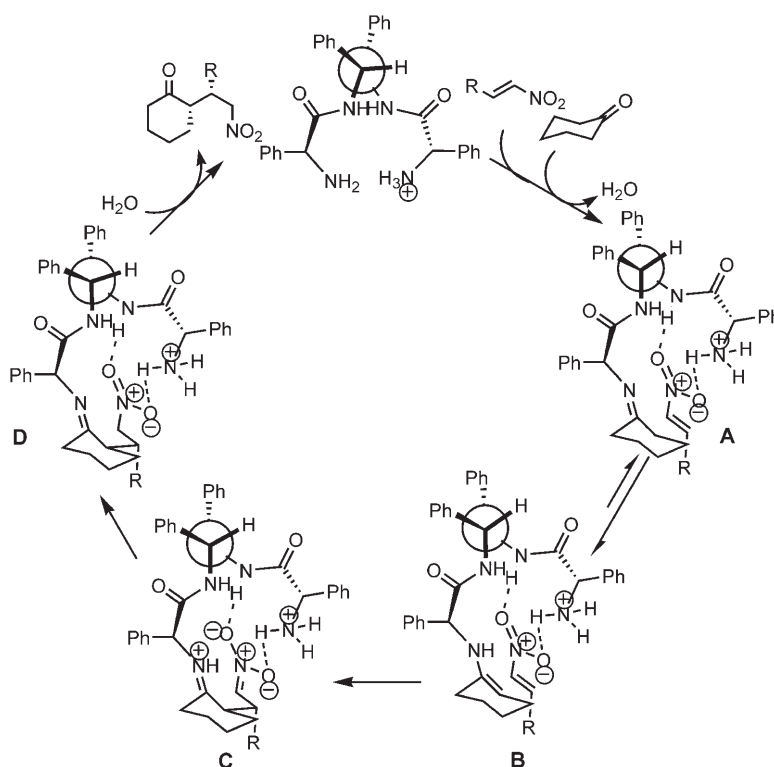
Figure 7. The proposed mechanism (anion \text{TsO}^- was omitted).
