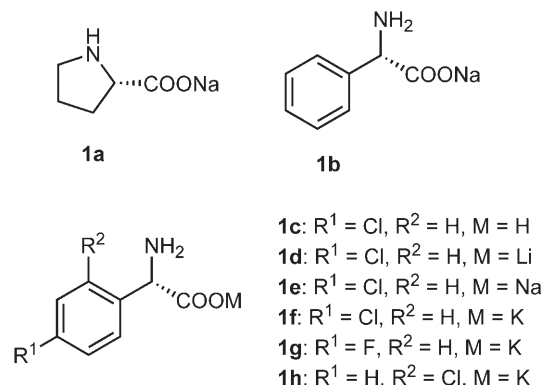
Figure 3. The evaluated chiral anion catalysts.
