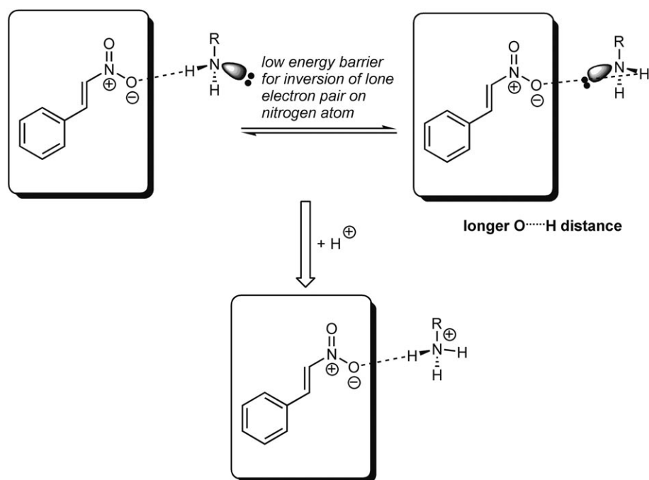
Figure 5. Proposed effect of the amine protonation process on the hydrogen bond.
